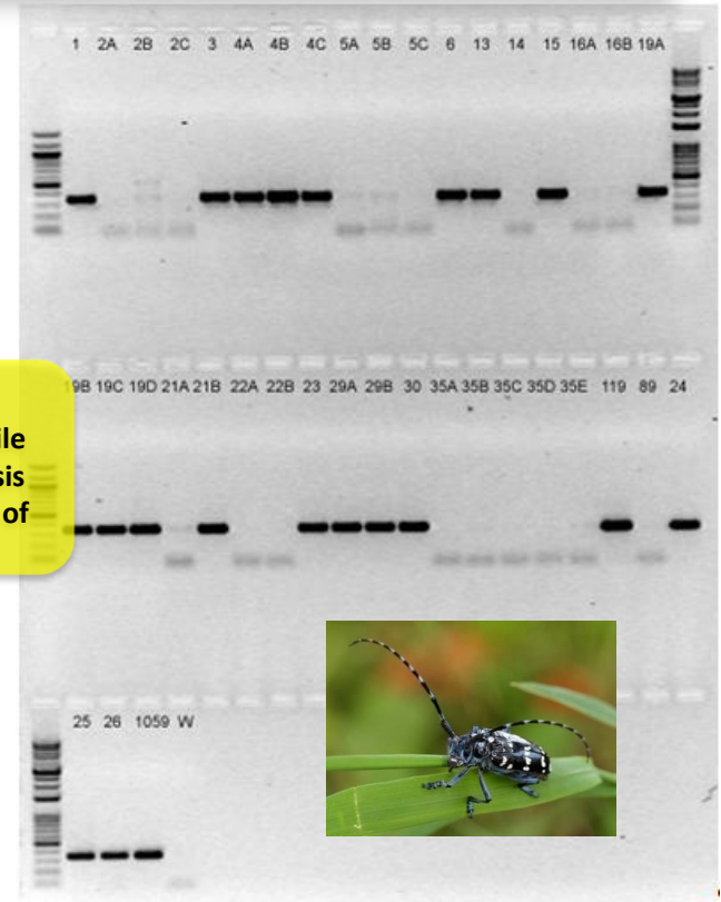
Figure 2 - Electrophoresis gel of amplified DNA fragments (primer ChinensisF/ChinensisR) from larval and pupal specimen, DNA diluted 1:100; A. bungii (89), A. chinensis adults (24, 25, 26), A. chinensis larva (1059), water (W). Molecular weight marker: Promega BenchTop 100bp DNA Ladder and PCR BIO Ladder I.
